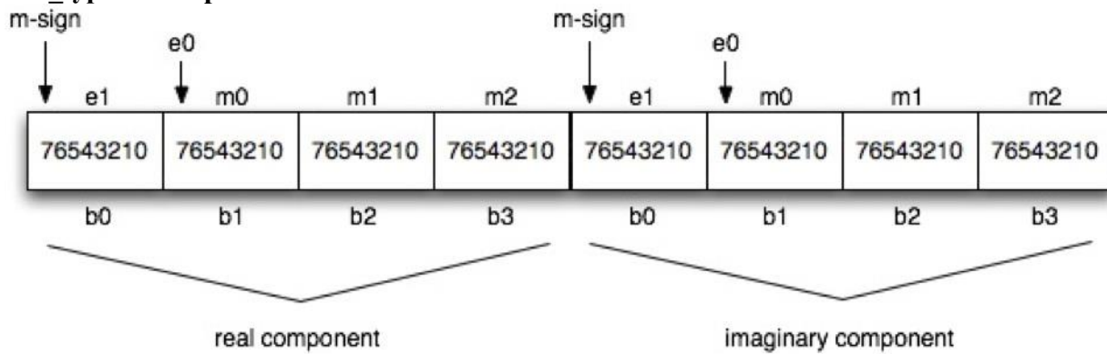
Fig. 5C-22. Single precision complex, most significant bytes first.
