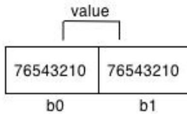
Fig. 5C-24. Unsigned bit string
