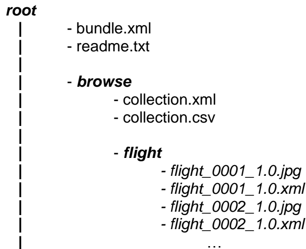
Figure 2B-1: Illustration of the structure for one browse subdirectory (one collection) with many basic products organized into sub-directories.
