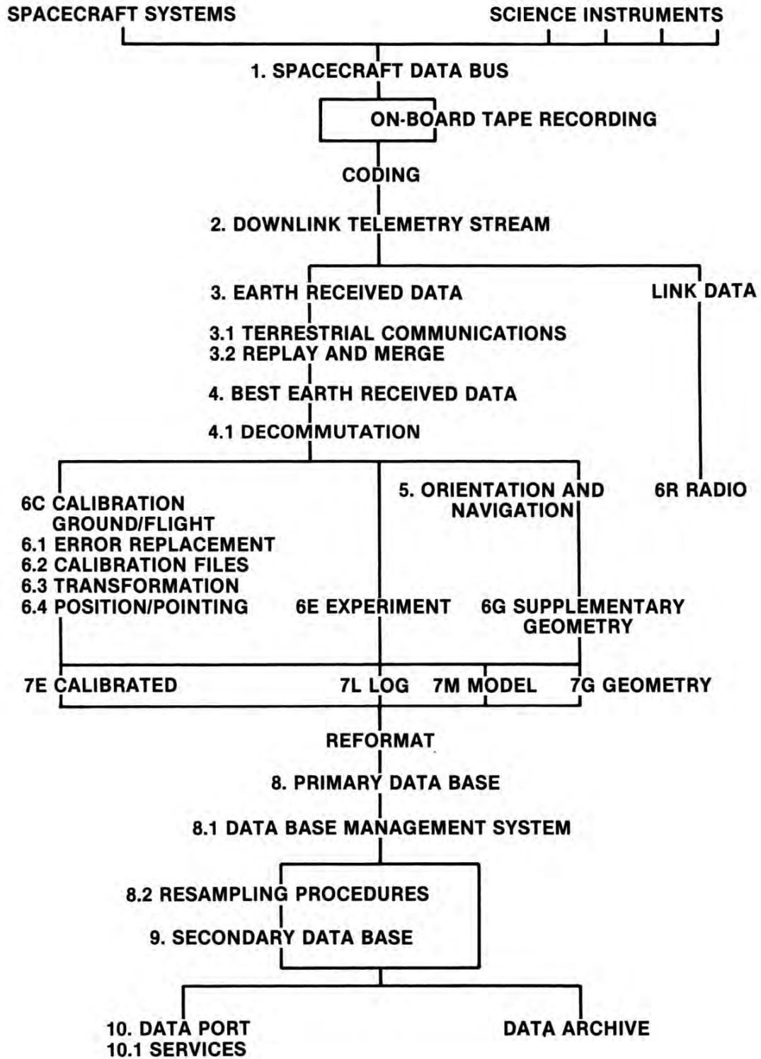
FIGURE 2.1 GENERAL DOWNLINK DATA FLOW
